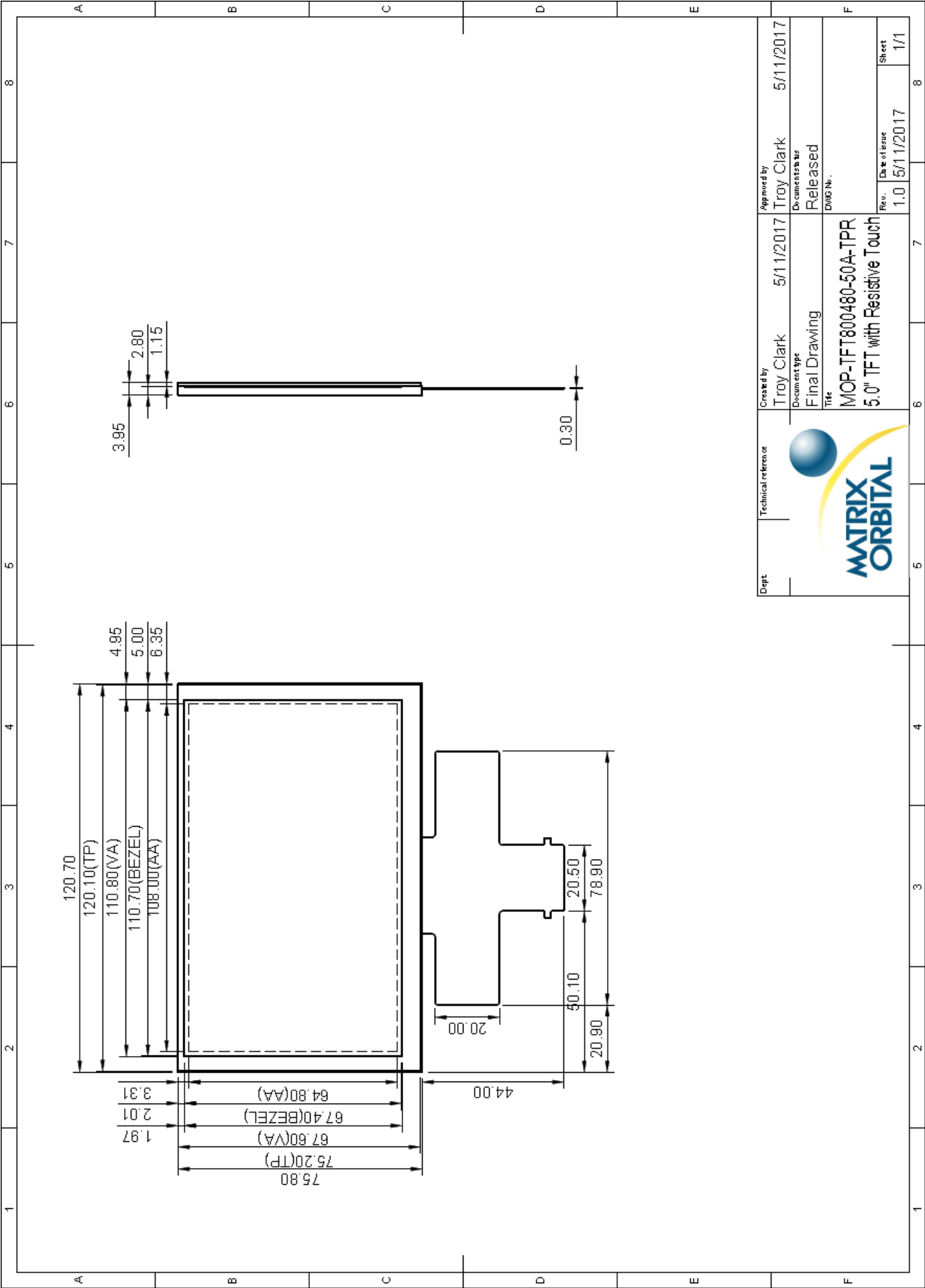
Figure 1: MOP-TFT800480-50A-BLM-TPR Drawing
